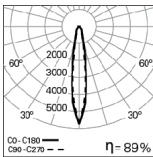
AXIS Sq/C 1 10W PB 4000K 14°
