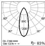
AXIS Sq/C 1 10W PB 4000K 36°
