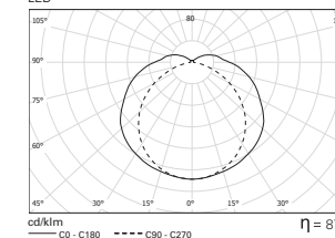
ECP LED 2x27W DC0 LED
