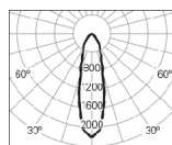
CO-C180 C90-C270 - - \eta = 85\% ELI Sq /E 1 PB 4000K 35°
