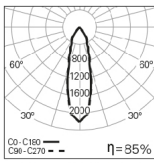
ELI Sq /W PB 4000K 35°
