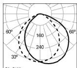
00-C180 C90-C270 - - \eta = 79\% HOLI Sq /AS Grand 15W LIGHT+ 4000K
