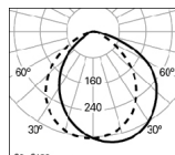
00-C180 C90-C270 - - \eta = 77\% HOLI Sq /AS Grand 20W LIGHT+ 4000K
