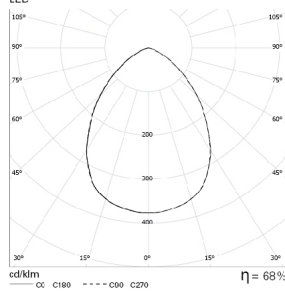
HOLI SQ Grand 17W DAM LED
