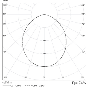
HOLI SQ Max 17W BLINE LED
