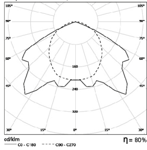
JUKE 1x18W PB Lamp: 1 x TC-DEL 18W/840
