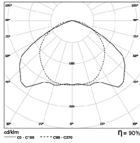
JUKE 1x26W PB Lamp: 1 x TC-TEL 26W/840
