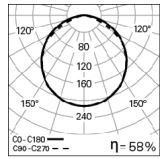
SLIM LED 11W DOZ 4000K
