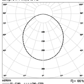
TEE 3x14W DOP Lamp: 3 x 14W/840 HE
