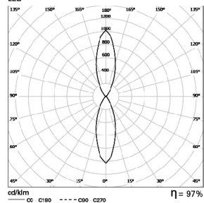
TREK /P LED 26W LED
