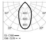
WEBB Spot /E 2 PB 4000K 60° HO
